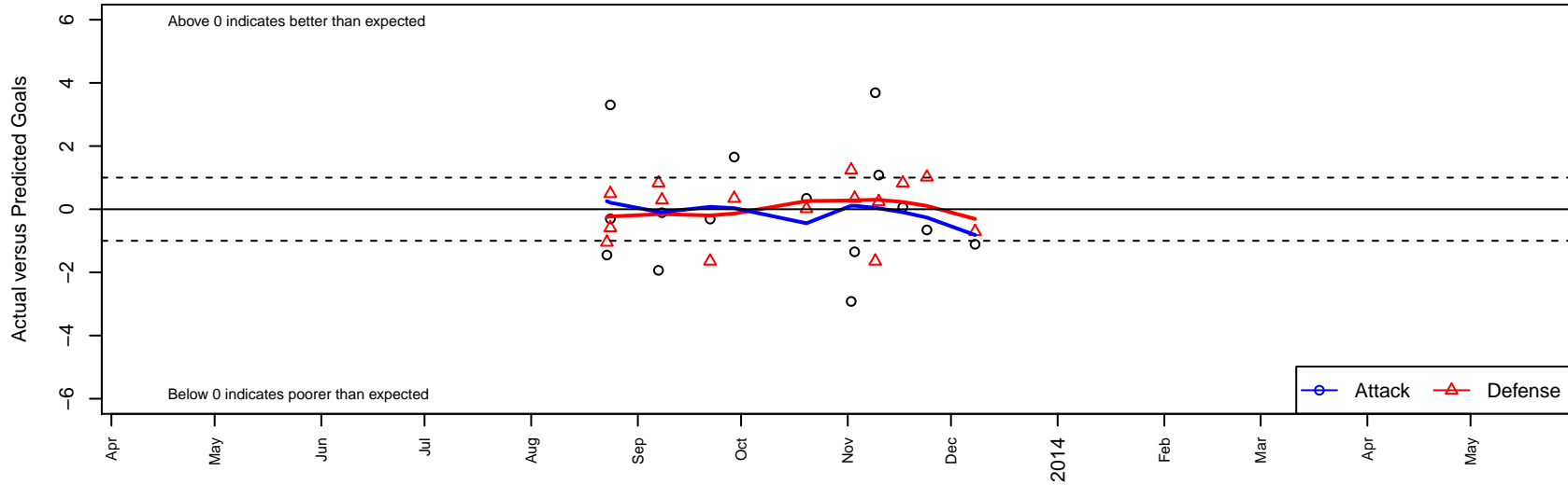
Wenatchee Fire Black B95 Dots are actual minus expected GF (blue circles) and GA (red triangles). Blue line is smoothed change in attack strength. Red is smoothed change in defense strength.
